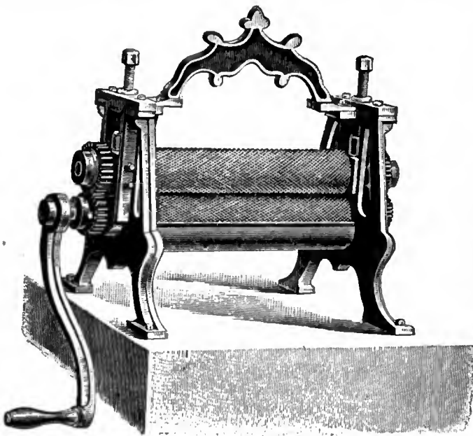
FIG. 23.—Foundation Machine (scale \frac{1}{2} ).
