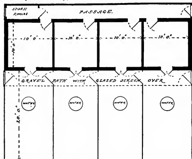
FIG. 2.—Plan of 4-compartment Aviary for Foreign Birds.
