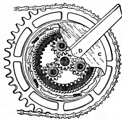
FIG. 13.—Sunbeam Two-Speed Gear.
