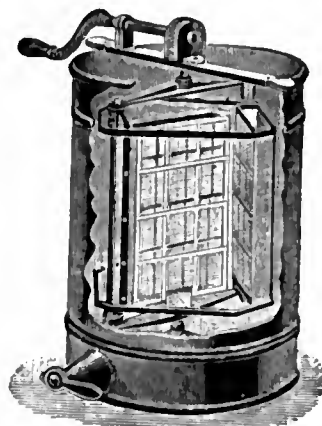
FIG. 20.—Cowan's rapid Extractor.
