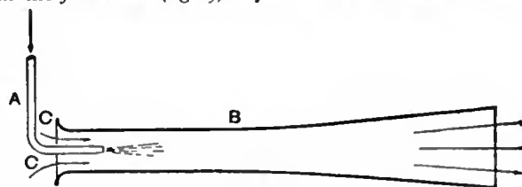
FIG. 9.—Steam-jet Blower.
