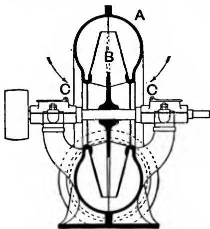
FIG. 8.—Günther's Blowing Fan.
